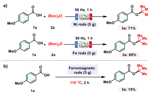
Scheme 4 The influence of metal in steel needles on the experimental results. Conditions: 1a : 0.5 mmol, 2a : 1.0 mmol, high temperature and pressure resistant reaction tube: 10 mL, Ni rods: 5 g, 1.0 × 5.0 mm, reaction time: 1 h, frequency: 50 Hz.
