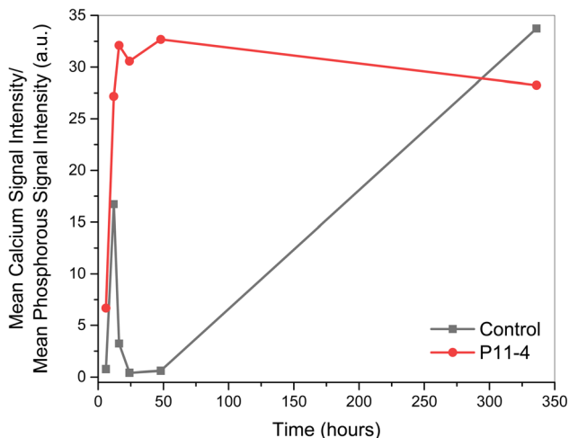
Fig. 7 Mean calcium-to-phosphorus signal intensity ratio against time, comparing the control to the SiN windows with deposited P 11-4 . The 400 μm × 400 μm map was split into eight regions, from which the calcium and phosphorus signals intensity was calculated. The mean signal intensity value of calcium and phosphorus was calculated from the eight regions, and the ratio of the values was plotted on the y-axis against time on the x-axis. The dark grey line indicates the values calculated for the control while the red line indicates the values in the presence of P 11-4 .
