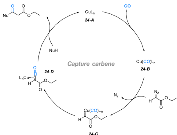
Fig. 24 Copper-catalyzed direct carbonylation of carbenes.
