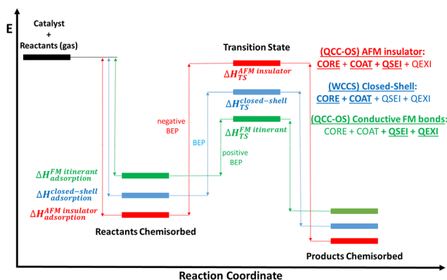
Fig. 2 In relation to the Bell-Evans-Polanyi (BEP) principle, the relative energy position of the transition states ( \Delta H^{\ddagger}_{TS} ) versus the reaction enthalpy ( \Delta H^{\text{step}} ) in QCC-OS is different from WCCS. 1 Typically, QCC-OS with conductive FM bonds optimize inter-atomic (non-local) QSEI and QEXI in quantum catalysts, showing positive BEP deviations. Although the opposite typically occurs, the worst catalytic activity is observed for the most insulating AFM phases (AFMI), specifically type-G, unless the surface of the topological material is conductive.
