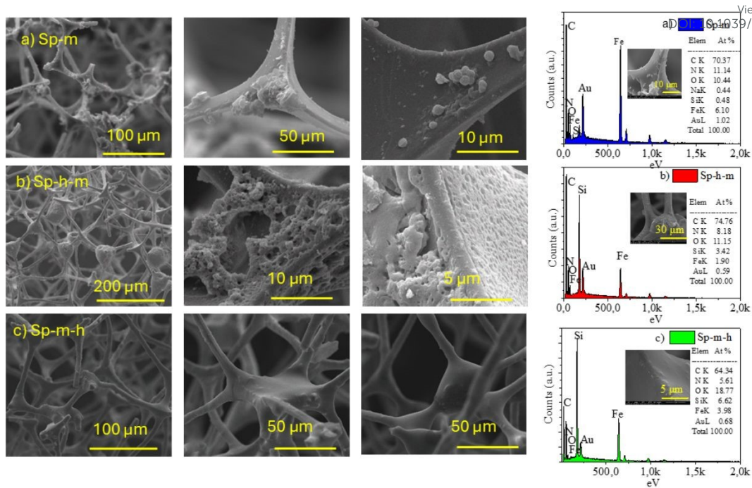
Figure 2. SEM images and the corresponding EDX spectra of the a) Sp-m, b) Sp-h-m and c) Sp-m-h samples.
