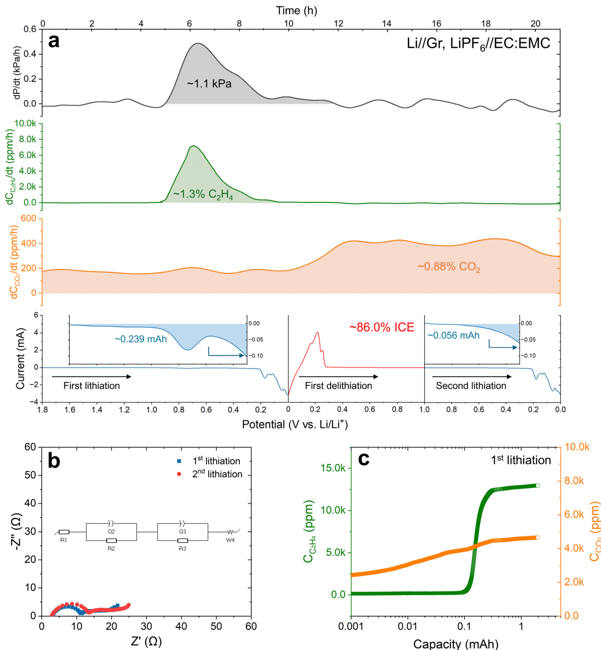
Fig. 5 Operando monitoring of gas evolution in the Li-graphite half-cell that undergoes cyclic voltammetry at a scan rate of 0.05 \text{ mV s}^{-1} with 1 \text{ M LiPF}_6 in EC : EMC 3 : 7 \text{ vol\%} as the electrolyte. (a) The obtained CV curves are plotted in conjunction with the change in concentrations of C_2H_4 , CO_2 , and in overall gas pressure. The detailed current variation from 1.8 \text{ V} to 0.3 \text{ V} vs. Li/Li^+ of the first lithiation and from 1 \text{ V} to 0.3 \text{ V} vs. Li/Li^+ of the second lithiation is provided in the insets by zooming in the y-axis. The blue shading of the first lithiation represents the electric charge consumed for the SEI formation and associated gas evolution. (b) The EIS spectra obtained after the initial and the second cathodic scan. (c) Evolution of C_2H_4 and CO_2 concentrations during the initial lithiation of graphite.
