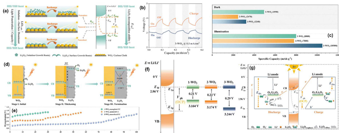
Fig. 24 (a) Schematic of the facet-controlled Li 2 O 2 growth routes and WO 3 photocatalytic activity in Li-organic PARBs, (b) photoresponses of the Li-organic PARBs with intermittent light on and off during both the discharge and charge processes for 3-WO 3 -nanosheet/CC, (c) galvanostatic discharge profiles of the three photocathodes at 50 mA g -1 without and with illumination, (d) Proposed mechanism for the photoassisted discharge, (e) long-term cycling test of the photocathode, (f) schematic band structure diagram for the prepared WO 3 /CC photocathodes, (g) schematic of charge/discharge process in the WO 3 /CC cathode under illumination. 85 Copyright: 2023 Royal Society of Chemistry.
