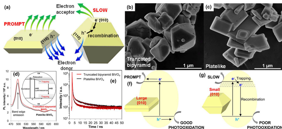
Fig. 25 (a) Schematic representation of facilitated charge transfer of large exposed {010} BiVO 4 surface. SEM micrographs of (b) truncated bipyramid and (c) platelike BiVO 4 , (d) steady-state fluorescence spectra of truncated bipyramid and platelike BiVO 4 (inset: mechanism of photoluminescence), (e) time-resolved PL spectra of the band-edge emission of truncated bipyramid and platelike BiVO 4 . 85 Copyright: 2016 American Chemical Society.
