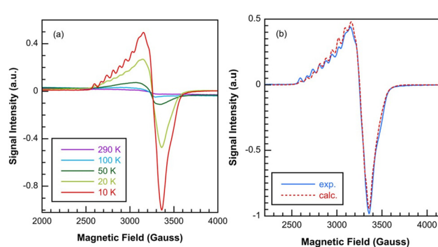
Fig. 9 (a) Thermal evolution of the X-band EPR spectrum of a \text{Cu}_4\text{L}_4 powder sample. (b) Experimental and theoretical EPR spectra at 4 K.
