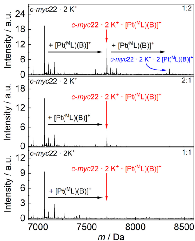
Fig. 7 Deconvoluted cryo-ESI-MS spectra of c-myc22 and [Pt(B)(M)L]OTf in DNA: complex ratios of 1:1 (bottom), 2:1 (middle) and 1:2 (top).
