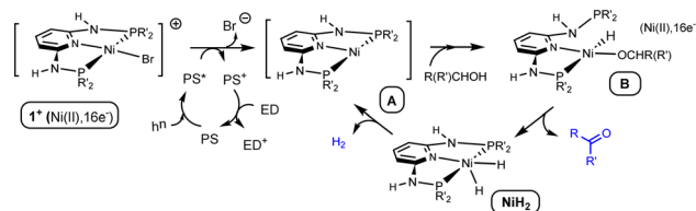
Scheme 4 Proposed mechanism for the photocatalytic molecular acceptorless dehydrogenation of alcohols with [Ni(2,6-(Ph 2 PNH) 2 (NC 5 H 3 ))Br] + . PS = Ru(bpy) 3 2+ , ED = DMEA.
