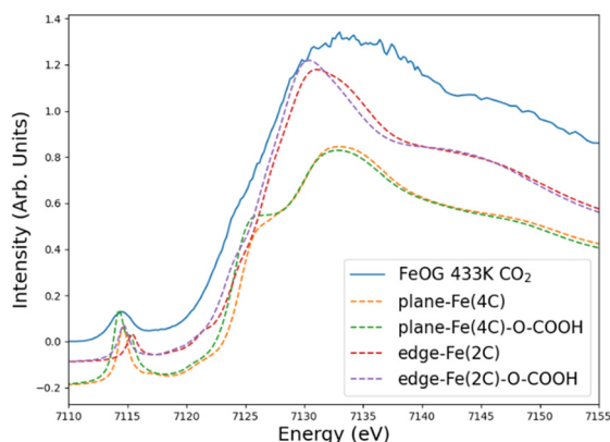
Fig. 7 Comparison between the XANES absorption spectrum of FeOG in CO 2 flow at 433 K (continuous line) and simulated XAS spectra (dashed lines) for a selection of Fe single atom centres. Spectra have been applied a vertical offset for clarity. Atoms in parenthesis specify the in-plane atoms binding Fe in the simulated structures.
