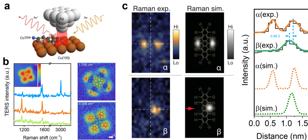
Fig. 53 Representative research work on TERS to achieve ultimate sensitivity and spatial resolution. (a) Schematic of TERS of the Co(II)-tetraphenyl porphyrin (CoTPP) molecule immobilized on Cu(100) in the LT-UHV TERS (6 K) system. (b) Spectra recorded on cobalt (1), pyrrole (2) and a phenyl group (3) are shown. The inset is the corresponding topography (left panel). The TERS mapping of Raman modes at 1156 \text{cm}^{-1} and 3006 \text{cm}^{-1} are shown (right panel). Scale bars are 2 Å. Reproduced from ref. 368 with permission. Copyright 2019 Springer Nature. (c) Measured and simulated maps for the C–H stretching mode of the pentacene species \alpha and \beta on the Ag(110) surface. Vertical and horizontal lines indicate the long and short molecular axes, respectively (left panel). Line profiles obtained along the short molecular axis. The orange and green curves are the Gaussian fitting of the peaks. Reproduced from ref. 370 with permission. Copyright 2021 AAAS.
