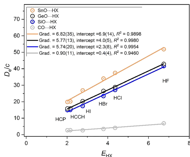
Fig. 2 Graphs of D_e/c versus E_{\text{HX}} for the four series MO \cdots HX (M = C, Si, Ge and Sn, and X = F, Cl, Br, I, CCH, and CP), in which the atom M adjacent to that (O) directly involved in the hydrogen bond belongs to Group 14.
