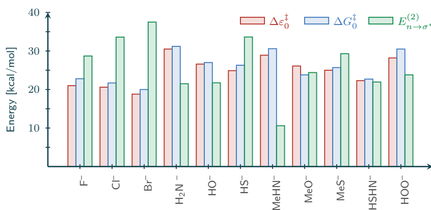
Figure 5: Electronic and Gibbs free intrinsic barriers, \Delta E_0^\ddagger , and second-order hyperconjugative stabilization energies, E_{n \rightarrow \sigma^*}^{(2)} for each nucleophile, computed at the MP2-SMD(THF)/cc-pVTZ level.
