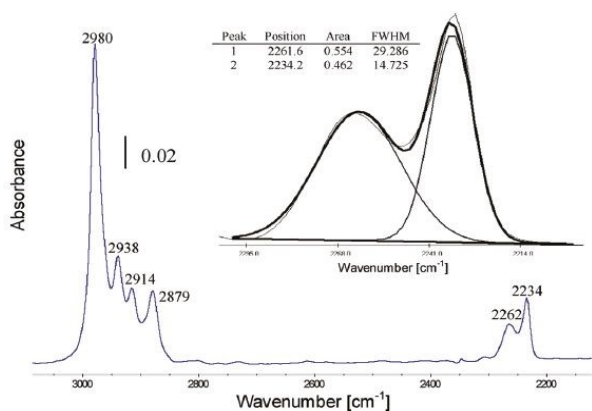
Fig. 17 tert-Butyl cyanide adsorption on carbonated MgO activated at 240 °C. The zoom-in region of 2300-2150 \text{cm}^{-1} . The deconvolution results are shown in the inset. Adapted from reference 4 with permission from American Chemical Society, copyright 2011.
