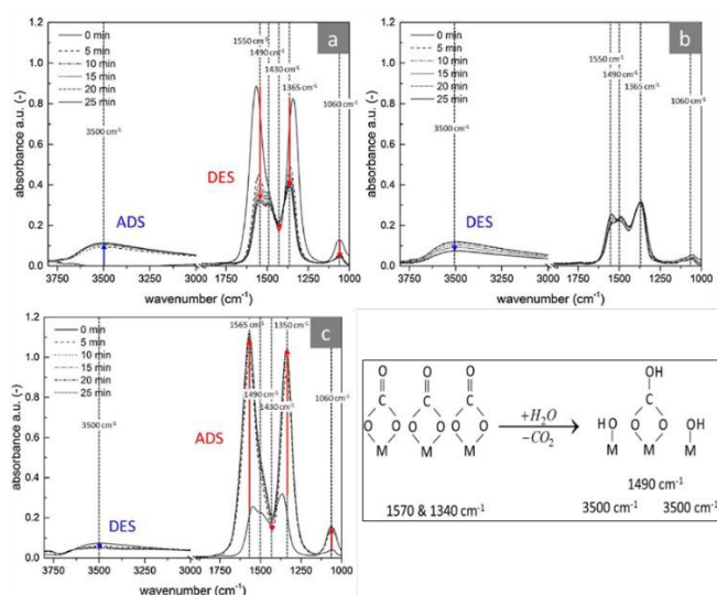
Fig. 15 IR spectra of hydrotalcite after (a) Adsorption of \text{H}_2\text{O} at 400 ^\circ\text{C} (b) Desorption of \text{H}_2\text{O} at 400 ^\circ\text{C} with \text{N}_2 (c) Adsorption of \text{CO}_2 at 400 ^\circ\text{C} after desorption with \text{H}_2\text{O} and \text{N}_2 . The equation shows \text{H}_2\text{O} adsorption and \text{CO}_2 liberation. Adapted from reference 1 with permission from Elsevier B. V., copyright 2018.
