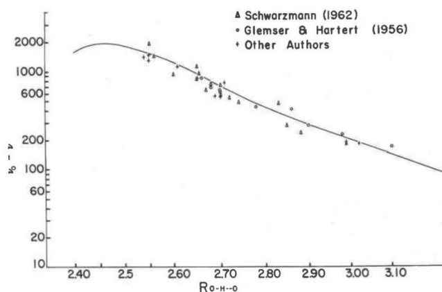
Fig. 9 Relationship between O-H frequency ( \nu ) and O-H...O distance in H-bonds ( R_{\text{O-H}\dots\text{O}} ); where \nu_0=3756 \text{ cm}^{-1} on the Y-axis. Adapted from reference 28 with permission from Mineralogical Society of America, copyright 1971.
