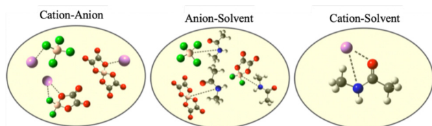
Fig. 2 Schematic of the interactions: cation-anion, anion-solvent, and cation-solvent.
