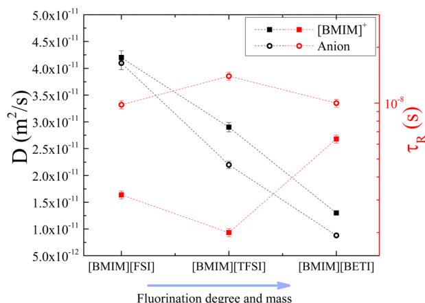
Fig. 8 Diffusion coefficients (black symbols) and rotational times (red symbols) of [BMIM]^+ (squared solid symbols) and the corresponding anion (circular hollow symbols) in the three ILs of group C, at 25 °C. Rotational times of [BMIM]^+ and [TFSI]^- in [BMIM][TFSI] are taken with permission from ref. 20. Dashed lines are guides to the eye.
