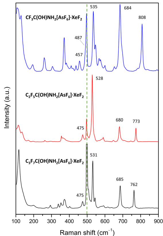
Fig. 8 Raman spectra of XeF_2 salt cococrystals with protonated amides recorded at low temperatures ( -90\text{ }^\circ\text{C} ). The green dashed line is placed at the position of free XeF_2 ( 497\text{ }cm^{-1} ) 41 which was observed as an impurity in the reactions.
