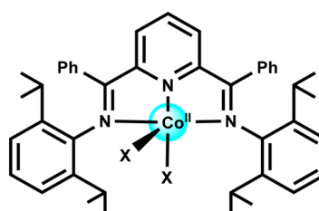
X = Cl ; Sq. Pyramidal, d = 0.57 Å, D = -72 cm -1 . X = Br ; Sq. Pyramidal, d = 0.54 Å, D = -67 cm -1 . X = I ; Sq. Pyramidal, d = 0.46 Å, D = -25 cm -1 .
