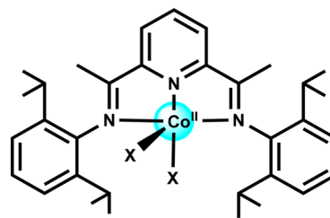
X = SeCN ; Sq. Pyramidal, d = 0.39 Å, D = -53.4 cm -1 . X = Cl ; Sq. Pyramidal, d = 0.55 Å, D = -55.4 cm -1 . X = Br ; Sq. Pyramidal, d = 0.54 Å, D = -32.1 cm -1 .
