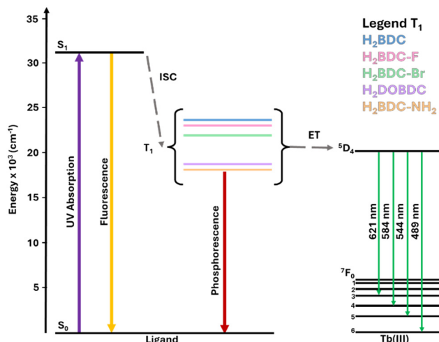
Fig. 6 Energy level diagram depicting the T_1 excited state for the linkers used to synthesize the various analogues of Tb(III)-UiO-66, highlighting the energy transfer from each linker to Tb(III), and the excited state energies of Tb(III).
