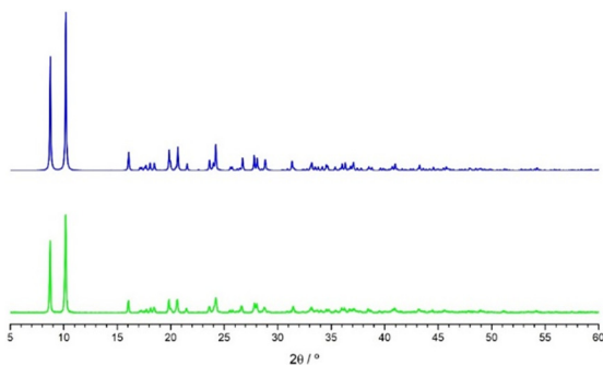
Fig. 2 PXRD diffractograms collected at \lambda ( \text{Cu K}\alpha_1 ) = 1.54056 Å of AgSD reported as SULPMS (green) experimentally obtained by the LAG method and simulated (blue).
