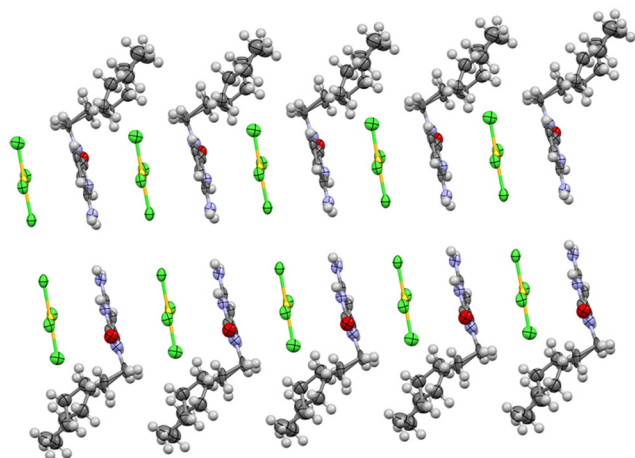
Fig. 6 View of crystal growing through the “b” axis, with anion- \pi interaction between cytosine rings and AuCl 4 displayed in the “a” direction.
