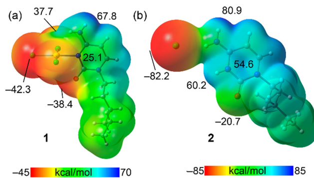
Fig. 8 MEP surfaces of compounds 1 (a) and 2 (b). MEP values at selected points in kcal mol -1 . Isovalue 0.001 a.u.
