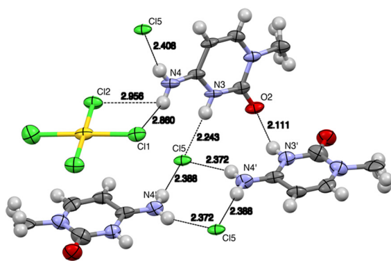
Fig. 7 View of the hydrogen bonds in the solid-state X-ray structure of complex 2. Distances in Å (aliphatic chains have been omitted for clarity). See Table 2 for the N...Cl distances with esd values.
