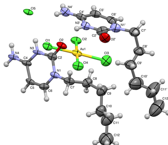
Fig. 5 View of asymmetric unit of X-ray structure for complex 2 . The aliphatic chain of one cytosine is disordered and have been solved over two positions ( \text{C}_7\text{A}-\text{C}_{12}\text{A} , 75% occupancy; \text{C}_7\text{C}-\text{C}_{12}\text{C} , 25% occupancy). The lower occupancy chain has been omitted for clarity.
