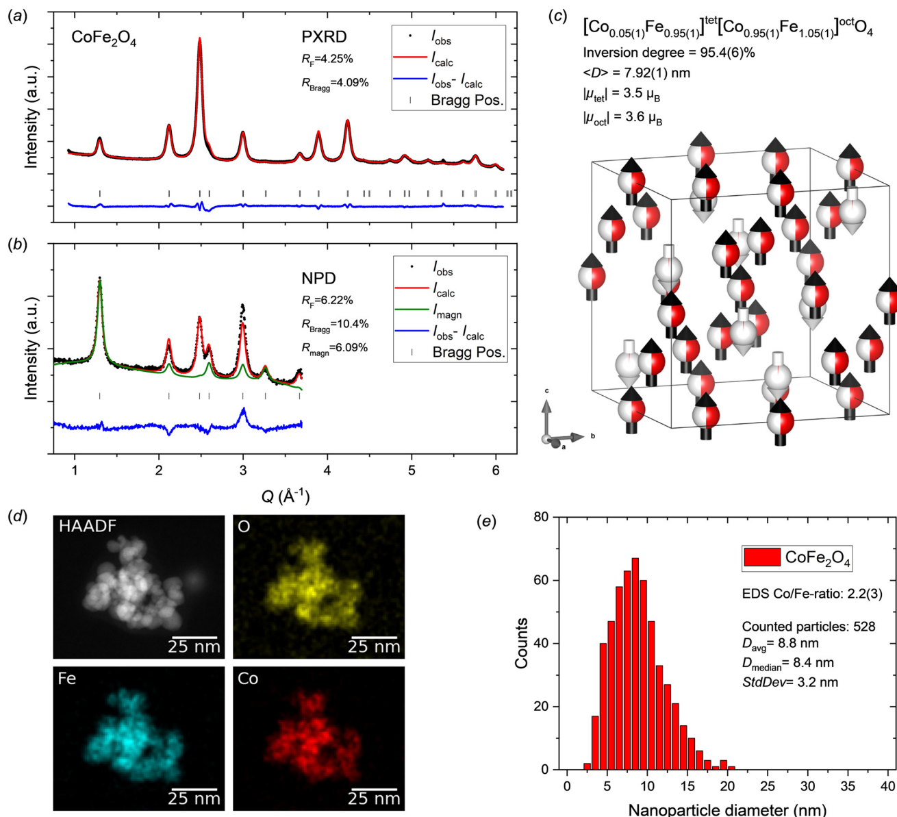
Fig. 3 a) PXRD and b) NPD data for CoFe 2 O 4 nanocrystallites with jointly refined Rietveld fits. c) Illustration of the refined crystal and magnetic structure of the CoFe 2 O 4 sample. The white and black arrows indicate the relative magnitudes and orientations of the refined magnetic moment components on tetrahedral and octahedral sites, respectively. The refined atomic site occupation fractions of Co 2+ (red) and Fe 3+ (white) are illustrated on the spheres. Illustration made with VESTA. 26 d) STEM-HAADF image and EDS elemental maps for the CoFe 2 O 4 nanoparticle sample. e) CoFe 2 O 4 nanoparticle size analysis from STEM data.
