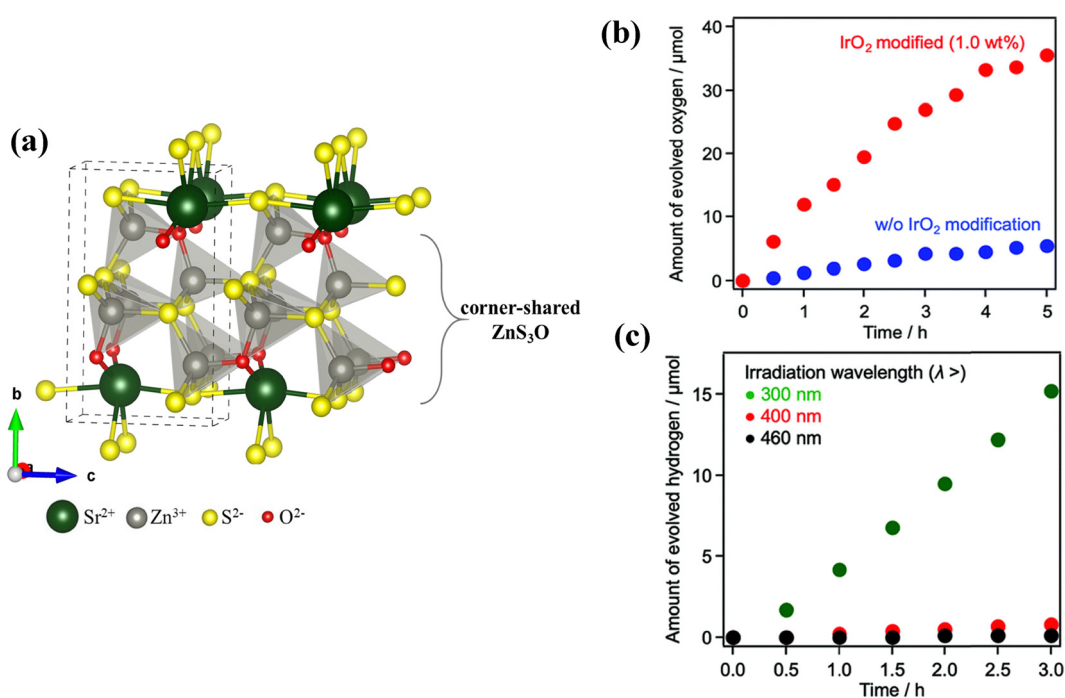
Fig. 4 (a) Structural representation of SrZn 2 S 2 O oxysulfide of Pmn 2 1 symmetry; (b) oxygen evolution for SrZn 2 S 2 O and (c) hydrogen evolution for Pt/SrZn 2 S 2 O. Reproduced from ref. 92 with permission from the Royal Society of Chemistry.
