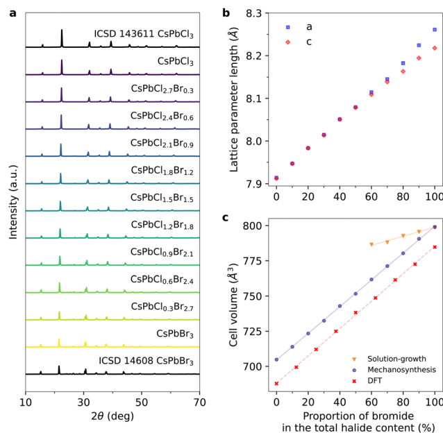
Fig. 2 (a) Powder XRD patterns of the mechanosynthesised CsPb(Cl x Br 1-x ) 3 samples. (b) Dependence of lattice parameters a and c on halide content in the mechanosynthesised powders. (c) Dependence of the cell volume on halide content in CsPb(Cl x Br 1-x ) 3 samples prepared by solution growth and mechanosynthesis, respectively. DFT-relaxed cell volumes for a set of special quasirandom structures 11 (SQS) are shown for comparison and confirm the Vegard-like behaviour; the overall shift is due to a typical slight overbinding of the particular DFT functional.
