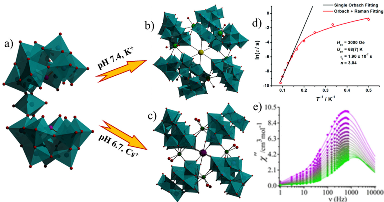
Fig. 3 The reaction conditions for the formation of [\text{K}\{\text{AsW}_9\text{O}_{33}\}\text{Dy}(\text{H}_2\text{O})_2\text{O}_6]^{35-} (b) and [\text{Cs}\{\text{Tb}_4(\text{H}_2\text{O})_8(\alpha\text{-AsW}_9\text{O}_{33})_4\}]^{23-} (c) from [\text{As}_2\text{W}_{19}\text{O}_{67}(\text{H}_2\text{O})]^{14-} (a) and their corresponding magnetic relaxation plot (d) and frequency-dependent out-of-phase magnetic susceptibility plot (e). Color code: cyan octahedron \{\text{WO}_6\} , green Dy, red O, yellow K, violet Cs, pink As. Hydrogen atoms are omitted for clarity. Figures reprinted (adapted) with permission from ref. 97 and 101. Copyright (2022) American Chemical Society, and (2017) Royal Society of Chemistry, respectively.
