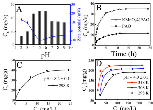
Fig. 4 Effect of pH on zeta potential of \text{KMnO}_4@\text{PAO} for \text{U}(\text{VI}) (A); effect of pH (A) and contact time on adsorption capability of \text{KMnO}_4@\text{PAO} for \text{U}(\text{VI}) (B); adsorption isotherms of \text{U}(\text{VI}) on \text{KMnO}_4@\text{PAO} and on PAO at \text{pH} = 8.2 \pm 0.1 (C) and at \text{pH} = 4.0 \pm 0.1 (D). m/V = 0.4\text{ g L}^{-1} , I = 0.1\text{ mol per L NaCl} . (A) T = 298 \pm 1\text{ K} , contact time: 24 h, C[\text{U}(\text{VI})]_{\text{initial}} = 20\text{ mg L}^{-1} , \text{pH} = 8.2 \pm 0.1 . (B) T = 298 \pm 1\text{ K} , C[\text{U}(\text{VI})]_{\text{initial}} = 20\text{ mg L}^{-1} , \text{pH} = 8.2 \pm 0.1 . (C) T = 298\text{ K} \pm 1\text{ K} , contact time: 24 h, \text{pH} = 8.2 \pm 0.1 . (D) Contact time: 24 h, \text{pH} = 4.0 \pm 0.1 .
