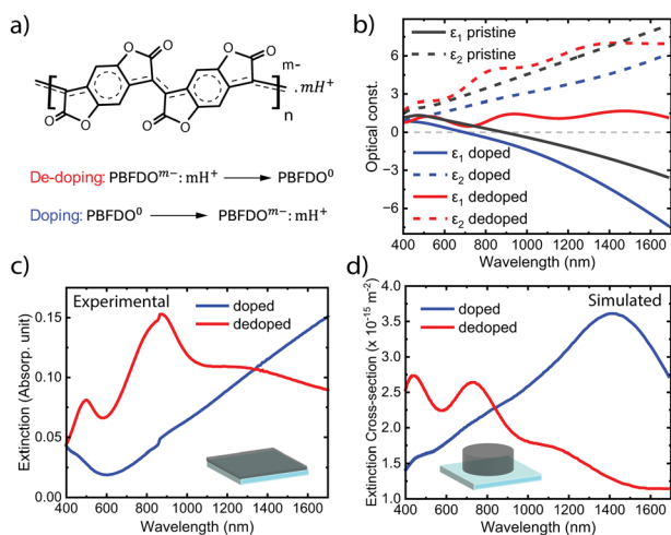
Fig. 1 (a) Chemical structure of n-doped PBFDO, and its doping/dedoping behaviour. (b) In-plane permittivity dispersion for PBFDO thin films in the pristine state (black), after doping (blue) and de-doping (red). Full lines correspond to the real component ( \epsilon_1 ) and dashed lines correspond to the imaginary component ( \epsilon_2 ). (c) Experimental extinction spectra of a PBFDO thin film (40 nm thickness) after chemical doping (blue) and dedoping (red). (d) Simulated extinction cross-section of a single PBFDO nanodisk on glass in its doped (blue) and dedoped (red) states (80 nm diameter, 30 nm height).
