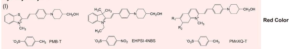
Fig. 2 Benchmark (a) and (b) non-ionic and (c)–(l) ionic organic THz crystals. For ionic organic THz crystals, there are four types of EDGs, either with or without intermolecular interaction capability: non-hydroxyl DA (4-(dimethylamino)phenyl) EDG, phenolic HM (4-hydroxy-3-methoxyphenyl) EDG, phenolic OH (4-hydroxyphenyl) and DH (3,4-dihydroxyphenyl) EDGs, and hydroxymethyl PM (2-(4-(4-(hydroxymethyl)piperidin-1-yl)phenyl)) EDG.
