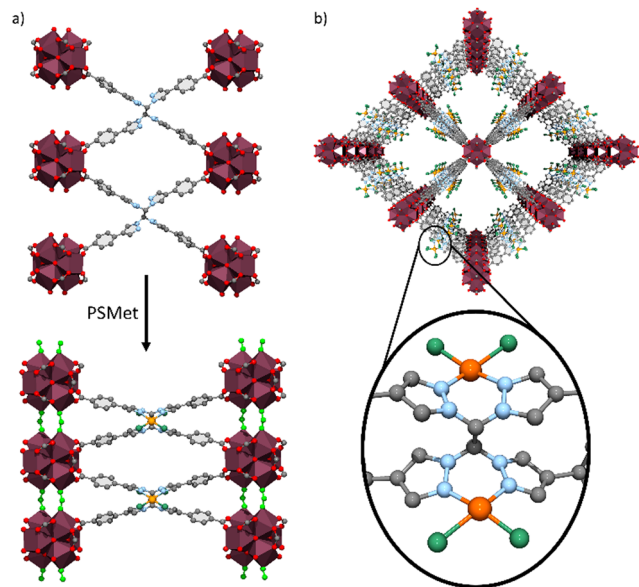
Fig. 5 (a) Representations of ligands bound to the Zr clusters in UAM-1002 (top) and UAM-1002[PdCl 2 ] (bottom). The transition from anti -(top) to syn -conformation (bottom) brings the Zr-clusters close enough that they end up being bridged by formate anions (represented in light green). (b) Representation of the structure of UAM-1002[PdCl 2 ] along the c axis, with the enlargement showing the PdCl 2 complex bound to the bis-pyrazole groups with a square planar geometry.
