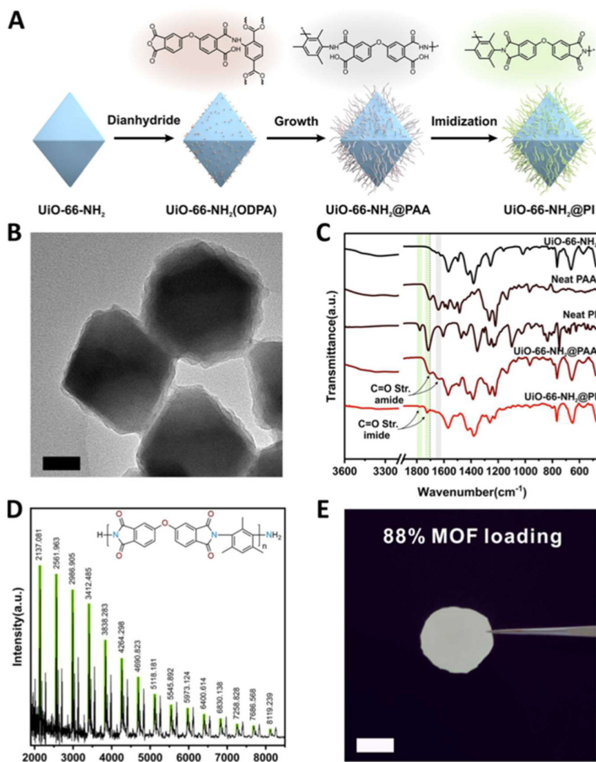
Fig. 6 (A) Synthetic procedure of making PI-grafted \text{UiO-66-NH}_2 . (B) TEM image of \text{UiO-66-NH}_2@\text{PI} . (C) FT-IR spectrum of the respective samples. (D) Mass spectroscopy results of grafted PI. (E) Photograph of a \text{UiO-66-NH}_2@\text{PI} -based PI membrane at 88% MOF loading. Reprinted with permission from Hongliang Wang, Sanfeng He, Xuedi Qin, Conger Li, and Tao Li. J. Am. Chem. Soc. 2018 140 (49), 17203–17210. DOI: 10.1021/jacs.8b10138. Copyright 2018 American Chemical Society.
