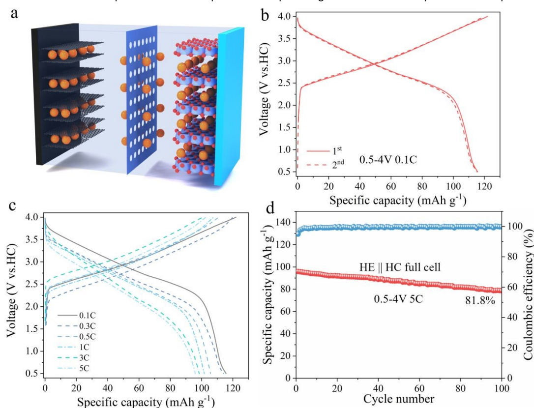
Fig.6 Electrochemical performance of HE full cell. (a) Schematic diagram of the full cell. (b) Charge-discharge curves of the material at 0.1C current density in the voltage range of 0.5-4 V. (c) Electrochemical curves of the material at different current densities. (d) Cycling plot of HE for 100 cycles under 5C conditions.
