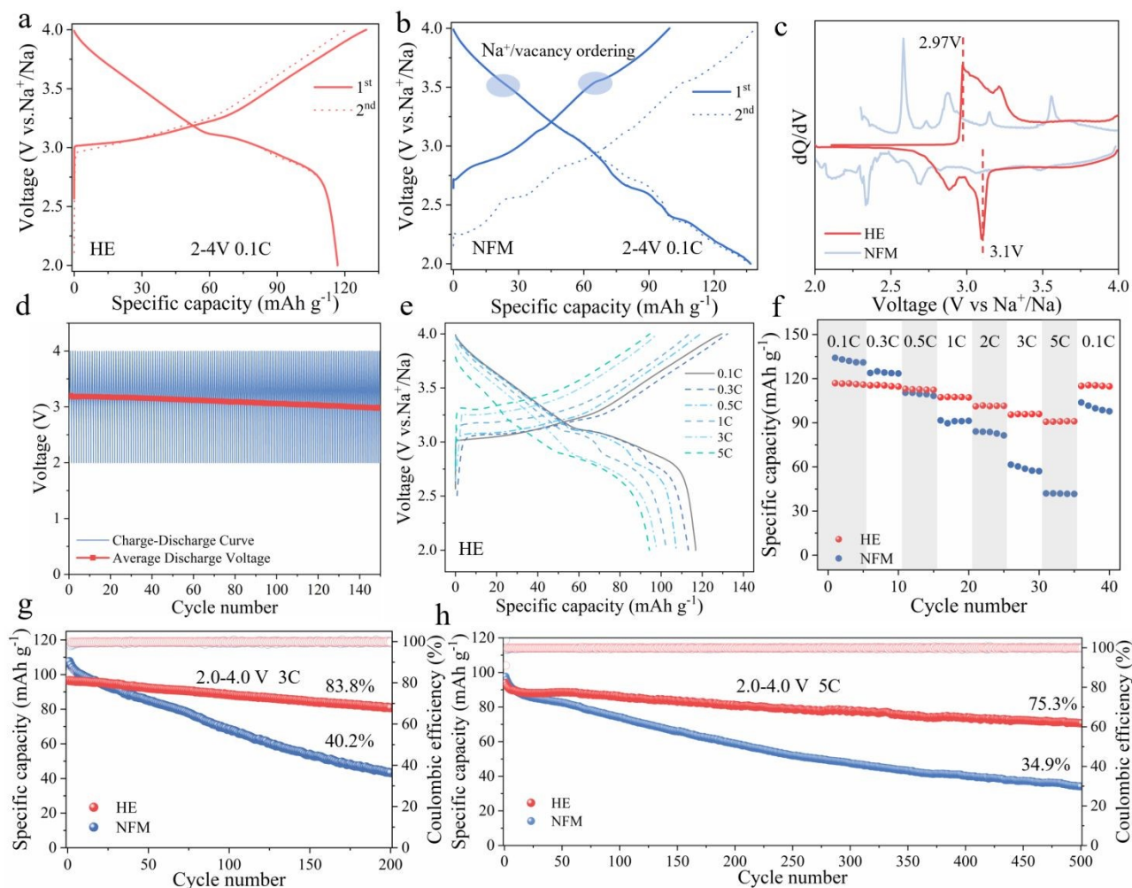
Fig.3 Comparison of electrochemical performance of electrode materials. First charge-discharge curves of (a) HE and (b) NFM at a current density of 0.1C within the voltage range of 2-4 V. (c) Comparison of dQ/dV curves. (d) The average discharge voltage variation of HE at 0.3C current density. (e) First charge-discharge curves of HE at different rates. (f) Comparison of rate performance of the materials. Cyclic performance of HE and NFM at (g) 3C and (h) 5C current densities.
