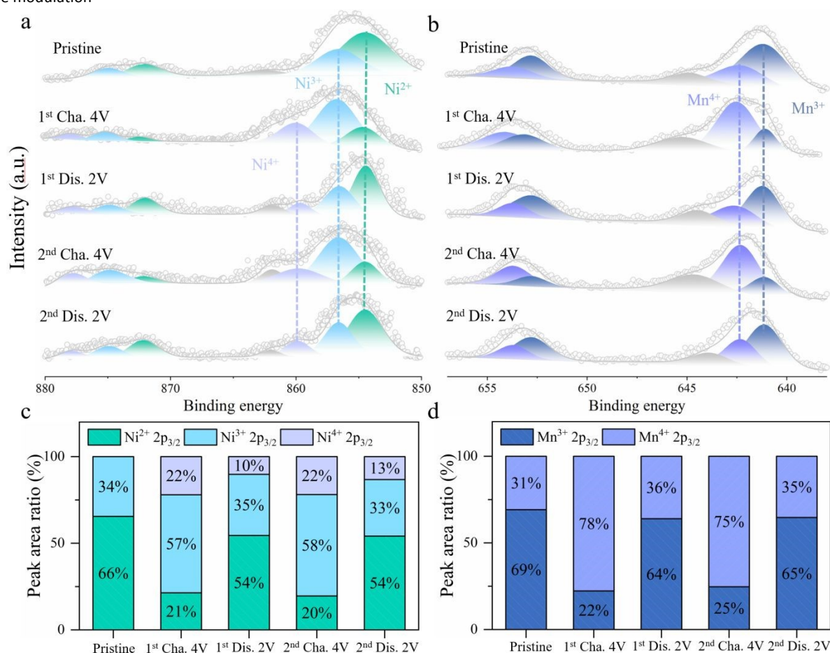
Fig.4 Redox mechanism of HE electrode material. (a) Changes in Ni 2p and (b) Mn 2p core spectra during the charge/discharge process, and the corresponding relative content changes of (c) Ni and (d) Mn in different valence states.
