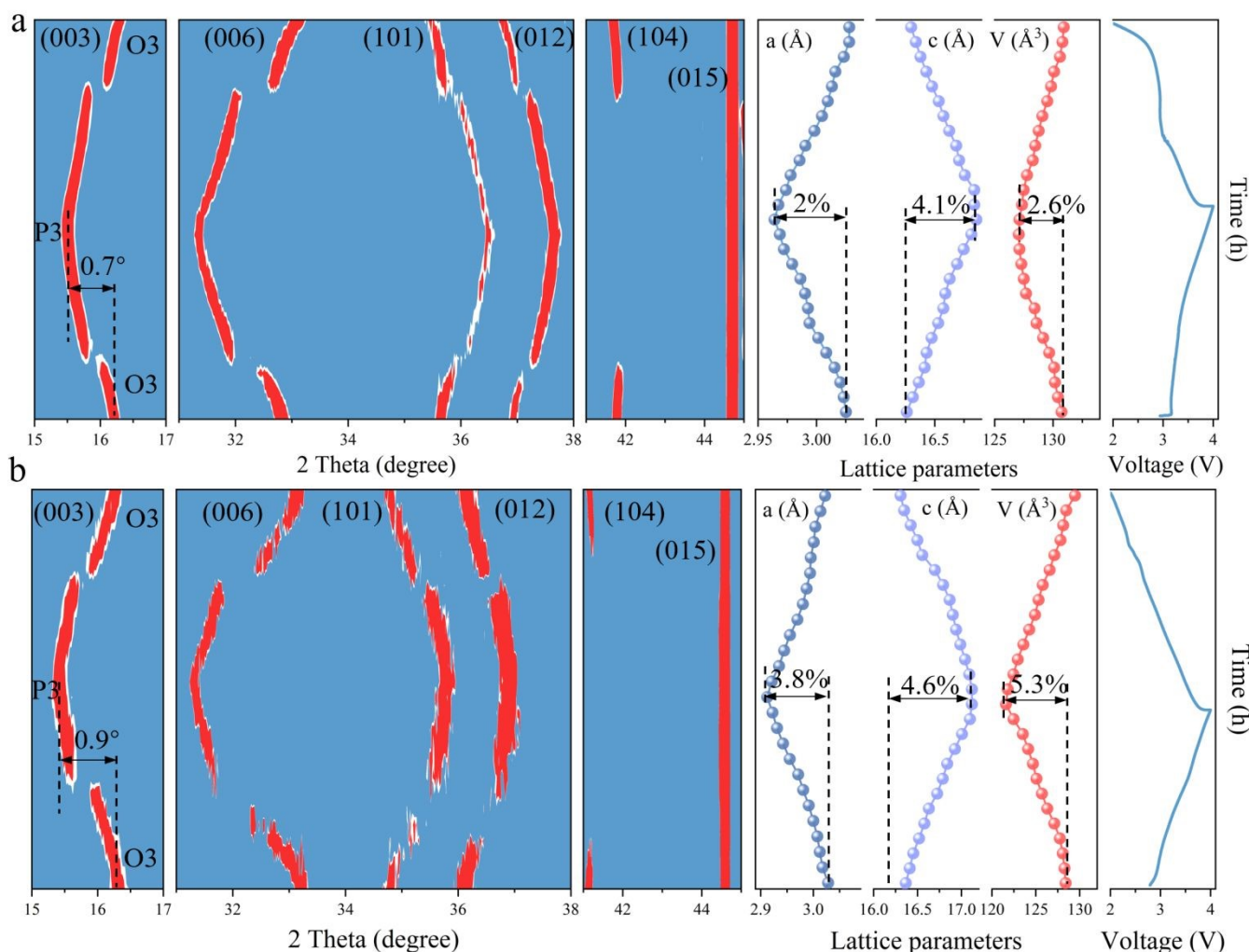
Fig.5 The structural evolution during \text{Na}^+ extraction/insertion. (a) The phase transition process of HE and the variation of lattice constants. (b) The phase transition process of NFM and the variation of lattice constants.
