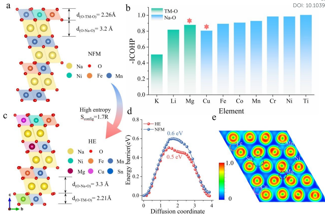
Fig.1 Structural comparison of NFM and HE materials. (a) The schematic crystal structure of NFM and corresponding interlayer distances between the sodium layer and TM layer. (b) Variation of bond strengths (TM-O and Na-O) in the Na-O-TM configuration after alkali metal and 3d transition metal substitution at the Mn site. (c) The schematic crystal structure of HE and corresponding interlayer distances between the sodium layer and TM layer. (d) The sodium ion migration barriers of NFM and HE. (e) The oxygen layer charge localization of HE.
