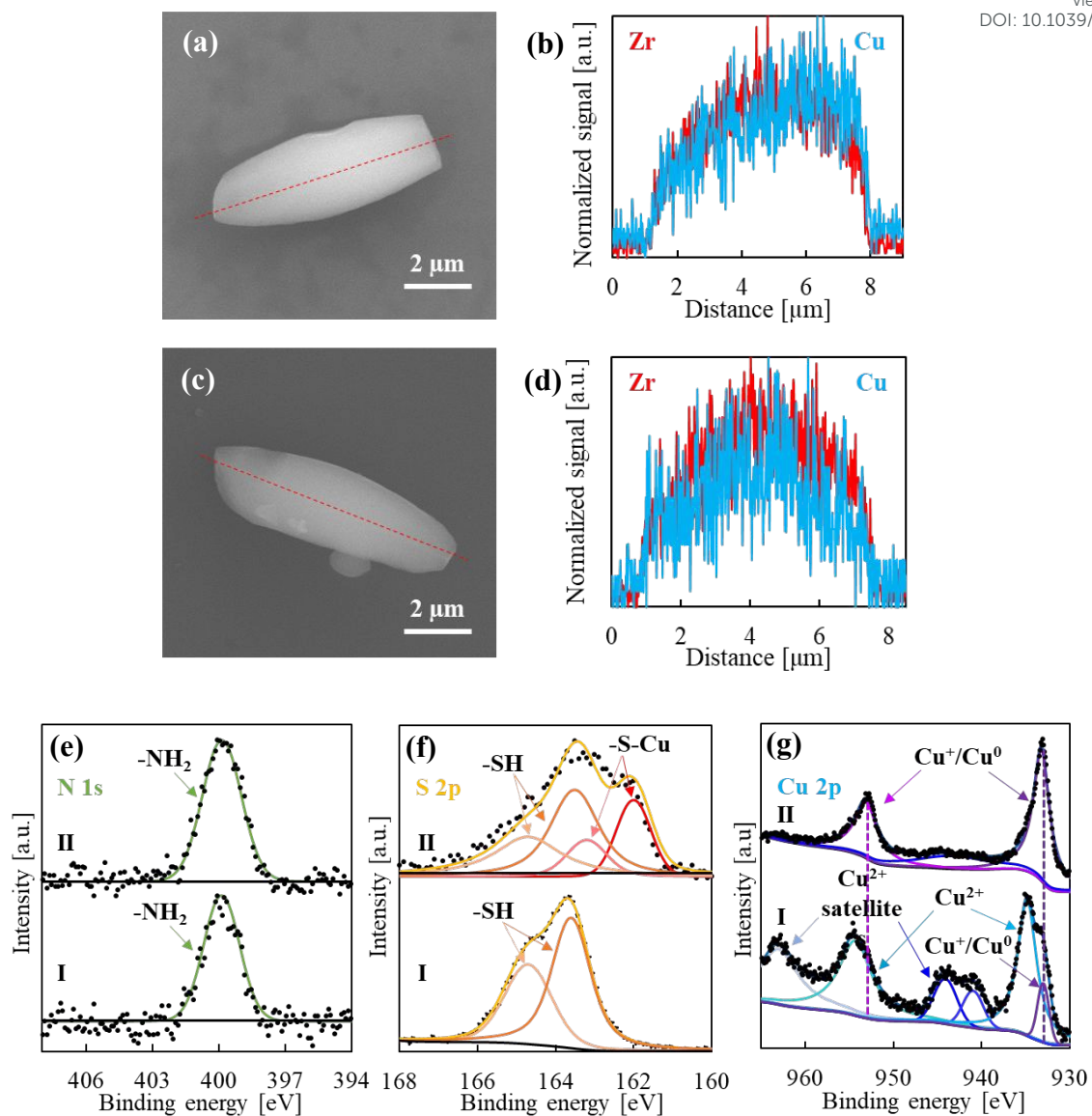
Figure 4. Characterization before and after thermal reduction: SEM images and Zr vs. Cu EDS line scans of (a,b) NU-1000-NH 2 /PrSH-Cu(For) 2 and (c,d) NU-1000-NH 2 /PrS-Cu, respectively; and XPS spectra of (I) NU-1000-NH 2 /PrSH-Cu(For) 2 and (II) NU-1000-NH 2 /PrS-Cu in the (e) N 1s , (f) S 2p and (g) Cu 2p regions, displaying the respective deconvoluted peaks.
