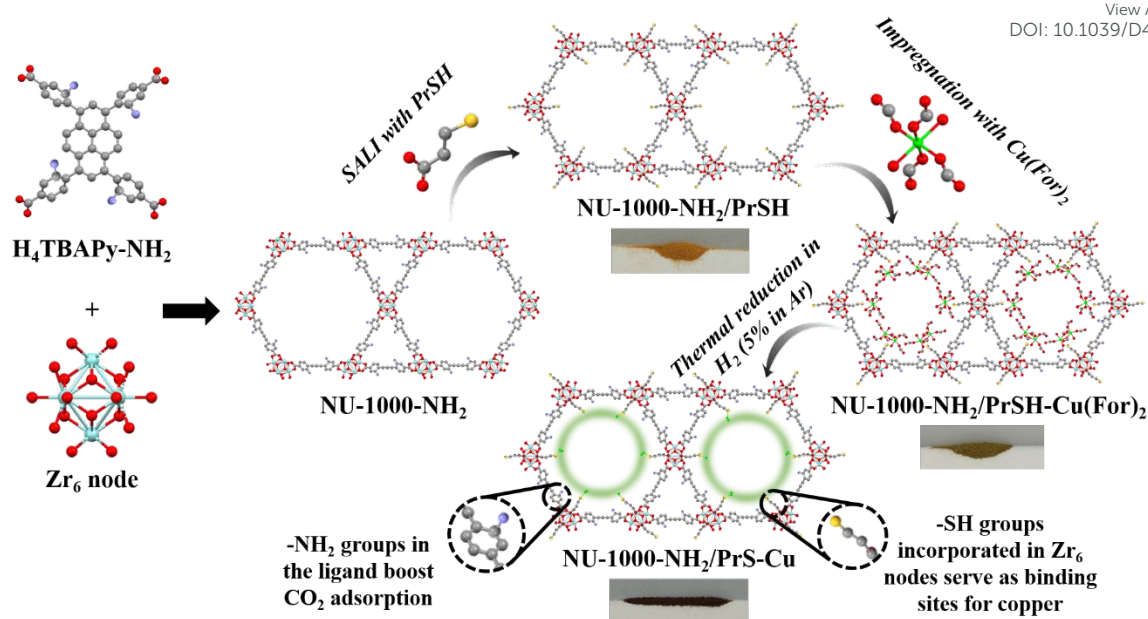
Figure 1. Schematic representation of the followed steps to synthesize NU-1000-NH 2 /PrSH-Cu, emphasizing in the purpose of the installed functionalities and including the color variation of the powder.
