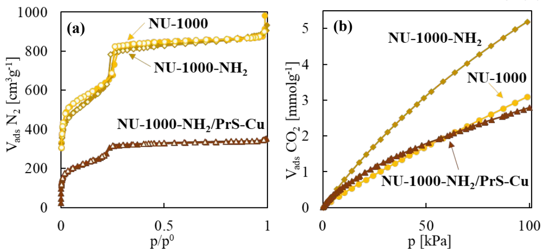
Figure 3. Adsorption behavior: (a) N 2 adsorption-desorption isotherms at -196 °C and (b) CO 2 adsorption isotherms at 0 °C of the studied samples compared to pristine NU-1000.
