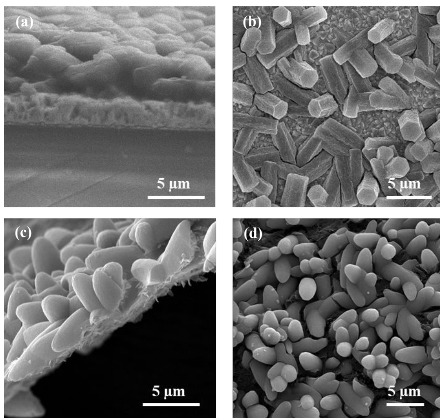
Figure 6. SEM micrographs of the samples tested for electrocatalysis: (a,b) NU-1000-NH 2 /PrS-Cu@FTO and (c,d) NU-1000-NH 2 /PrS-Cu@rGO taken from different angles.
