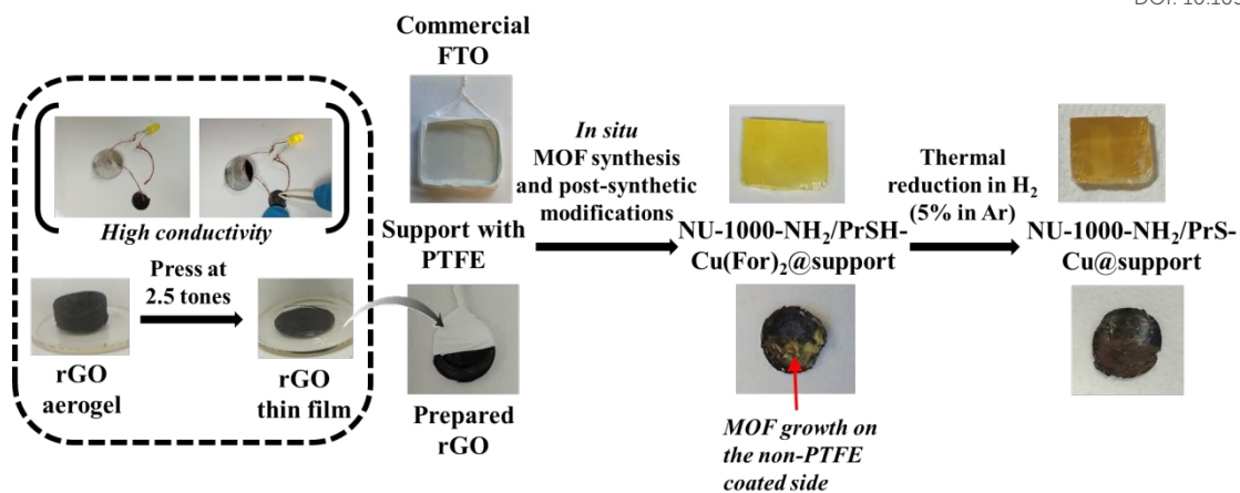
Figure 2. Schematic representation of NU-1000-NH 2 /PrS-Cu@support preparation.
