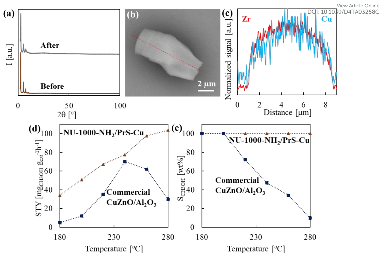
Figure 7. Characterization and results of the sample tested for thermocatalysis: (a) PXRD of NU-1000-NH 2 /PrS-Cu before and after testing, (b,c) SEM image and Zr vs. Cu EDS line scan of NU-1000-NH 2 /PrS-Cu after testing, and (d) MeOH space-time yield (STY) and (e) MeOH selectivity ( S_{\text{CH}_3\text{OH}} ) of NU-1000-NH 2 /PrS-Cu compared to commercial CuZnO/Al 2 O 3 at the different studied temperatures.
