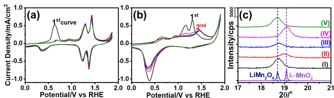
Fig. 2 The CV curves of the m -LMO-300-F2 electrode with a 5 mV s -1 sweep rate in neutral electrolytes of (a) 1.0 M LiNO 3 and (b) 1.0 M KNO 3 . (c) The XRD patterns of the m -LMO-300-F2 electrode before and after electrochemical measurements: (I) before cycling, (II) after sweeping from -0.1 to 1.7 V in the 3rd cycle in 1.0 M KNO 3 , (III) after reverse sweeping from 1.9 to 0.8 V in the 3rd cycle in 1.0 M KNO 3 , (IV) after sweeping from -0.1 and 1.7 V of the 1st cycle in 1.0 M LiNO 3 , and (V) after reverse sweeping from 1.9 to 0.8 V of the 1st cycle in 1.0 M LiNO 3 aqueous solution (bottom patterns are from the LiMn 2 O 4 and λ-MnO 2 references in ICDD cards, 00-054-0252 and 00-042-1169, respectively).
