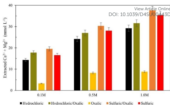
Figure 13: Combined calcium and magnesium extraction from mineral acid series dissolution, compared to single acid dissolution
