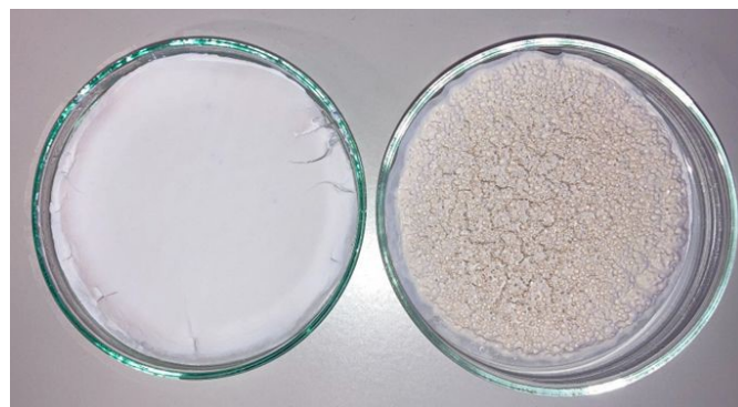
Figure 17: Carbonate filter cakes produced from calcite hydroxide experiments at 3 bar (left) and 9 bar (right)
