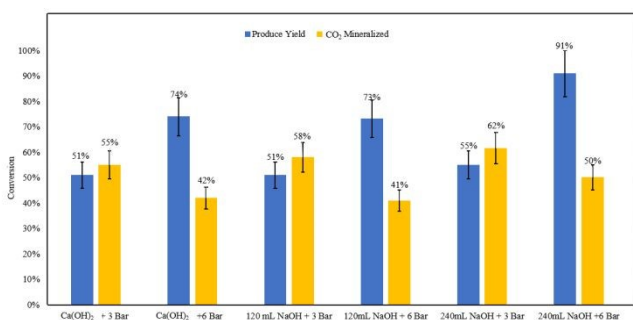
Figure 18: Measured product yields and \text{CO}_2 mineralization quantities based on mineral carbonation experiments
