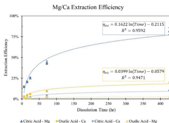
Figure 4: Effect of dissolution time in 0.5 M citric and oxalic acid solutions on Mg and Ca extraction
