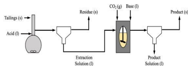
Figure 1: Process Flow Diagram for pH Swing Process
