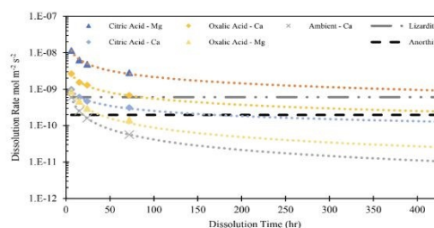
Figure 14: Measured Dissolution Rates based on release of Mg and Ca in 0.5M citric and oxalic acid solutions. Compared to measured Ca release rate and steady state anorthite dissolution, both at ambient temperature/pressure and pH=4.19 10,32
