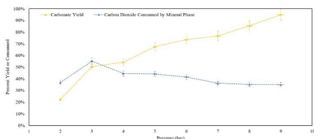
Figure 15: Percent yield of the residues and percent of CO 2 mineralized from what was provided to the reaction in the pressure varied calcite formation trials
