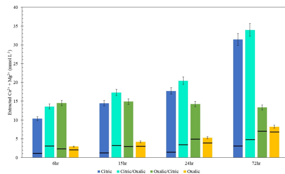
Figure 11: Combined calcium and magnesium extraction from acid series dissolution, compared to single acid dissolution, where the black bar represents the split between calcium (bottom) and magnesium (top)
