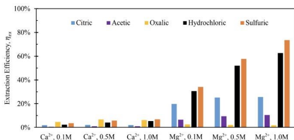
Figure 3: Extraction Efficiencies of All Acids at 0.1 M, 0.5 M, 1.0 M, overnight dissolution
