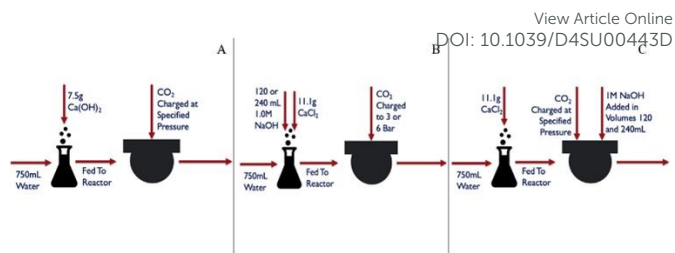
Figure 2: Experimental reaction pathways: (A) pressure variation experiments of calcium hydroxide carbonation; (B) ex-situ base addition carbonation of calcium chloride solution; and (C) in-situ base addition carbonation of calcium chloride solutions
