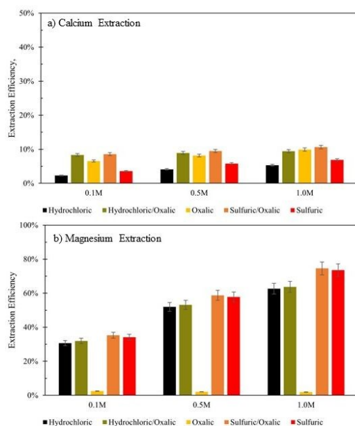
Figure 12: Extraction efficiency of (a) Ca 2+ and (b) Mg 2+ in mineral acid series dissolution, compared to single acid dissolution. Data organized by the solution concentration step of the series. Naming convention refers to the order of the acid(s) used
