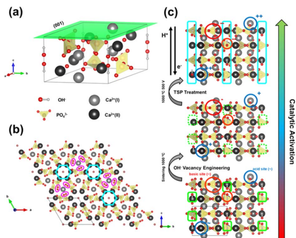
Scheme 1 Structure of HAP as a catalyst. (a) HAP unit cell P6_3/m . (b) (001) crystallographic plane observed from the c -axis direction. The \text{OH}^- channels and the Ca(II) 6-fold coordination are highlighted. (c) Structural changes and lattice refinement strategies adopted to achieve the catalytic activation of HAP.
