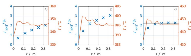
Fig. 3 \text{NH}_3 molar fraction measured at distinct sampling position (blue) and spatially resolved temperature profile (red) at temperature levels of 350 °C (a), 400 °C (b) and 450 °C (c). Reaction conditions: \text{H}_2/\text{N}_2 = 3.0 and pressure of 80 bar using the Fe catalyst.
