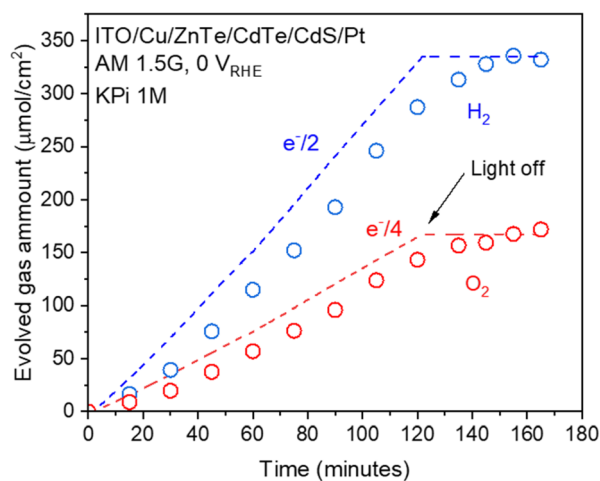
Fig. 10 Hydrogen and oxygen evolution from the ITO/Cu/ZnTe/CdTe/CdS/Pt (RTA) photocathode under simulated sunlight in a three-electrode configuration with an applied potential of 0 V_{RHE} . The expected amounts of hydrogen and oxygen (denoted as e^-/2 and e^-/4 , respectively) as calculated from the observed photocurrent are shown as dashed lines. A 1 M aqueous KPi solution with pH adjusted to 6.5 with KOH was used as the electrolyte.
