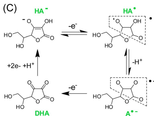
Scheme 2 (A) Possible mechanisms for the light-driven \text{H}_2 production with the system Ru/Co/HA - /H 2 A (Ru = Rubpy or RuSPphen). (B) Diagrams of potentials referred versus SCE for the redox couples of RuSPphen and Rubpy PSs at the ground and excited states, the [Co(CR14)Cl 2 ] + (Co) catalyst, and HA - . (C) Oxidation processes of ascorbate salt (HA - ) to dehydroascorbic acid (DHA) and back reduction of DHA to HA - .
