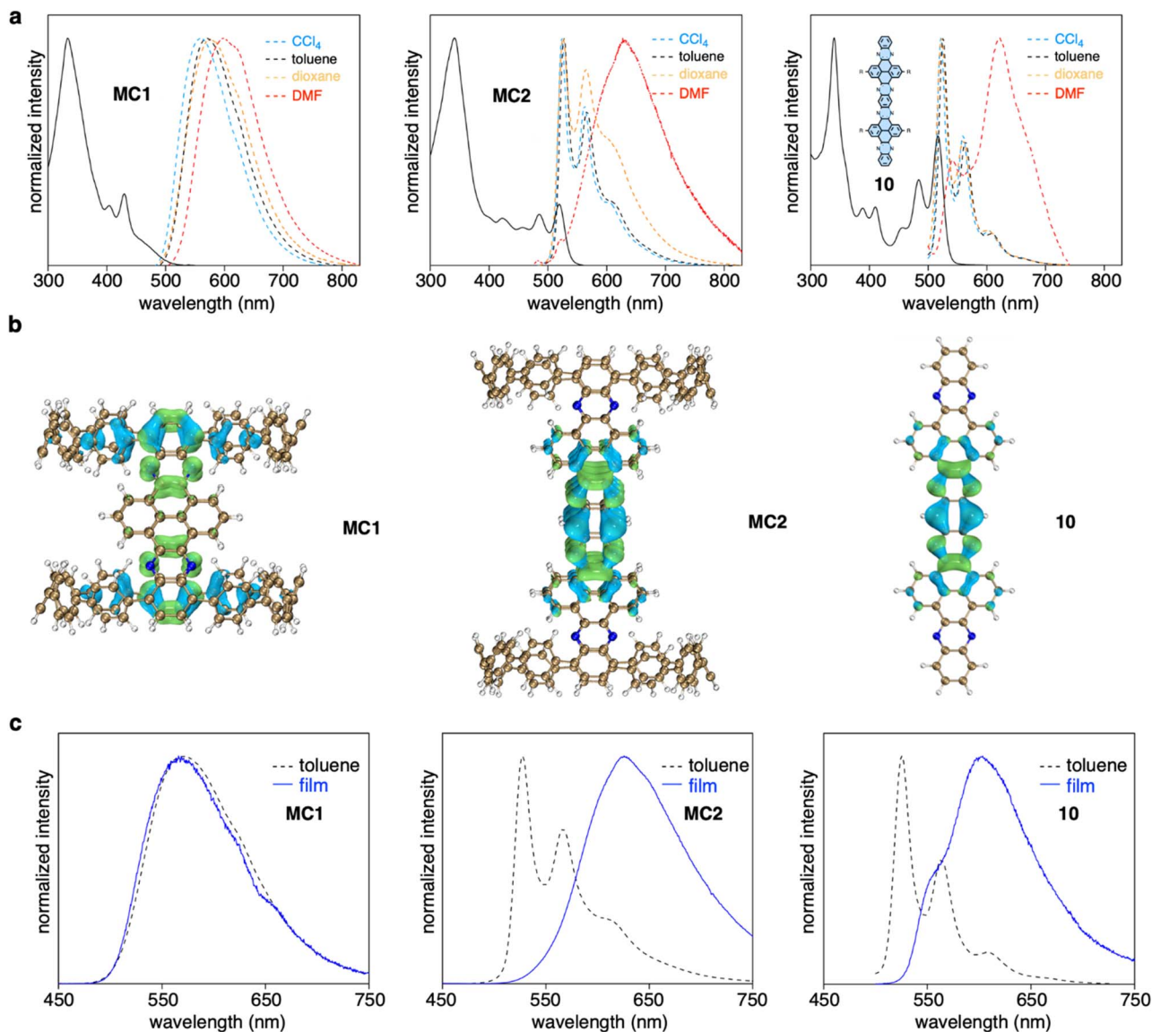
Fig. 4 Photophysical properties. (a) UV-vis absorption (solid line) and fluorescence (dashed line) spectra of MC1 , MC2 , and 10 . (b) Electron-hole analysis of the S_0 \rightarrow S_1 excitation. Blue and green regions denote hole and electron distributions, respectively (isovalue = 0.001). (c) Fluorescence spectra measured in toluene solution and in the film state.
