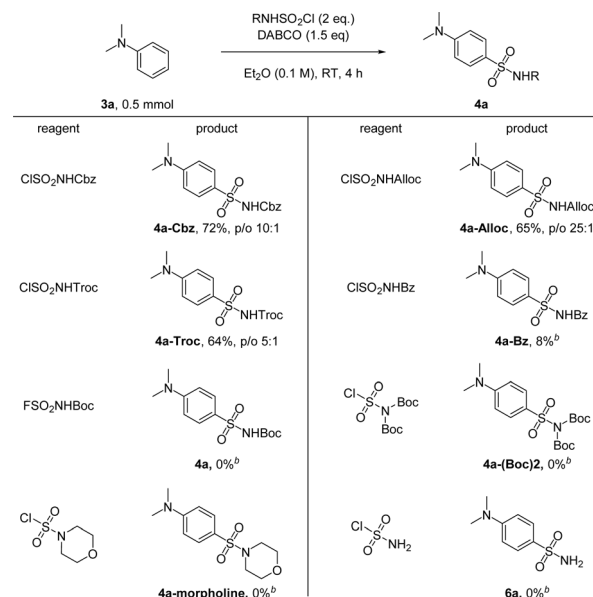
Scheme 5 Reaction of 3a with other N -sulfonylamine precursors. Cbz = CO 2 CH 2 Ph, Alloc = CO 2 CH 2 CH=CH 2 , Troc = CO 2 CH 2 CCl 3 , and Bz = C(=O)Ph. [b] 0.1 mmol scale.
