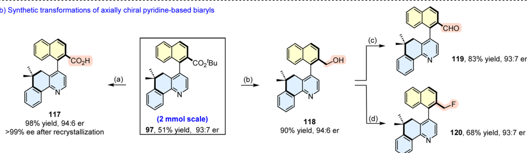
(b) Synthetic transformations of axially chiral pyridine-based biaryls
