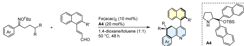
(a) Construction of axially chiral pyridine-based biaryls
