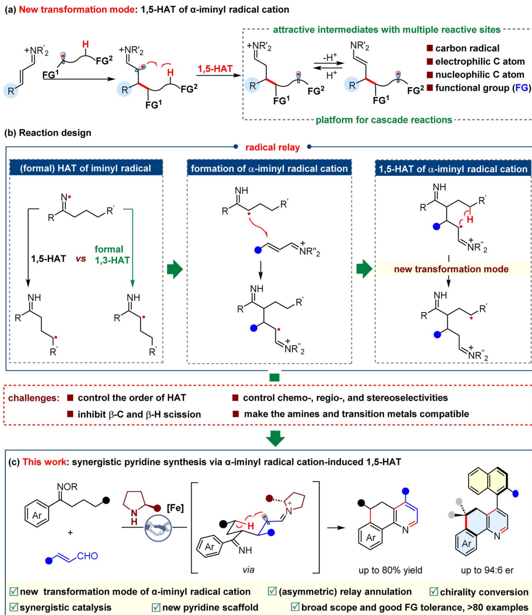
Scheme 2 Design plan based on \alpha -iminy radical cation-induced 1,5-HAT.
