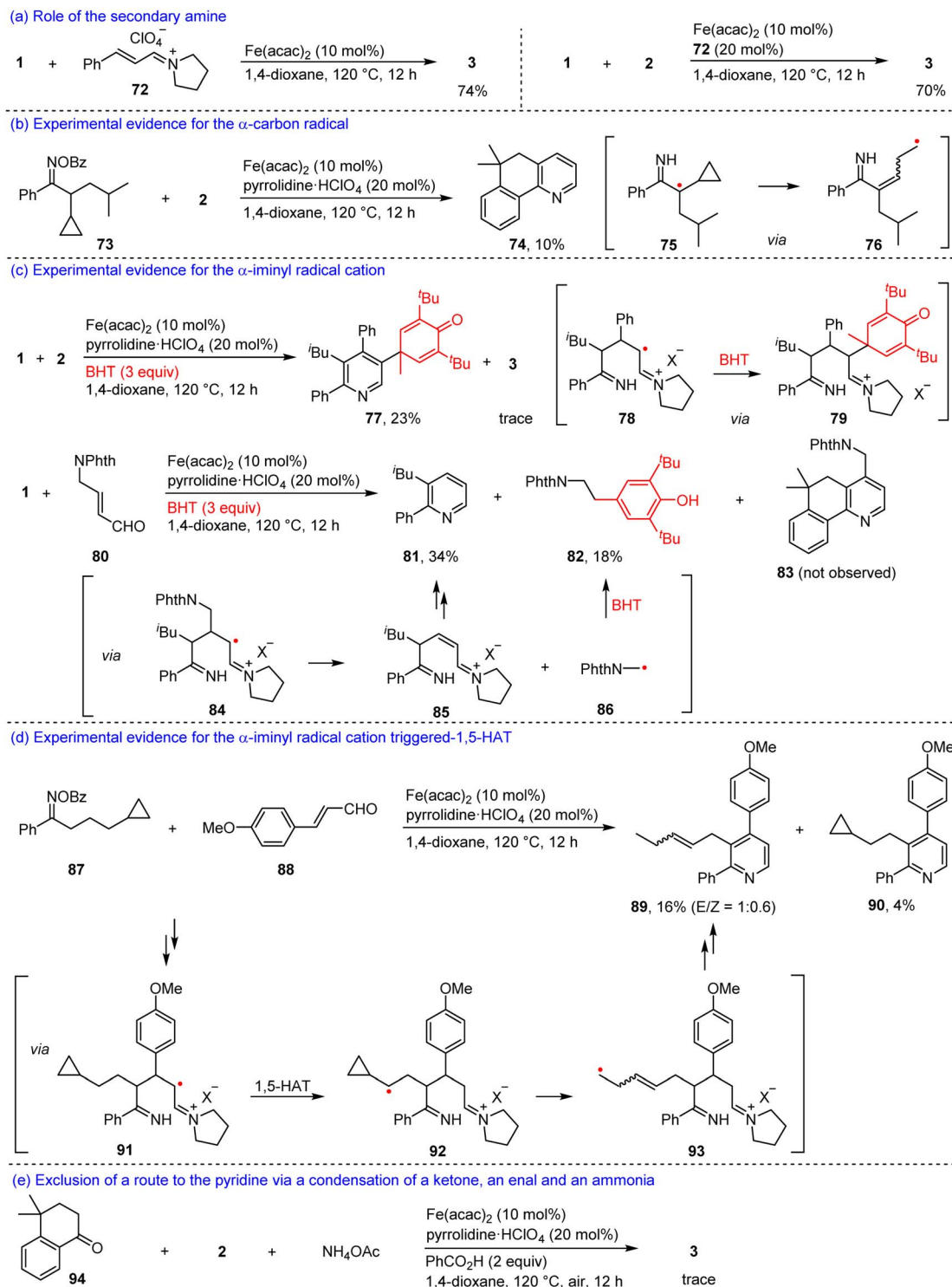
Scheme 6 Mechanistic studies ( X = \text{ClO}_4 , \text{OBz} , or \text{acac} ).
