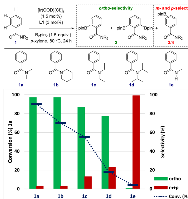
Fig. 4 Relevance of the steric parameters of the amide group in benzamides 1a–1e for the supramolecular iridium-catalysed C–H borylation. Reaction conditions: 1 (0.162 mmol), Ir(COD)(Cl) 2 (1.7 mg, 2.43 × 10 −3 mmol), L1 (4.1 mg, 4.86 × 10 −3 mmol), B 2 pin 2 (61.7 mg, 0.243 mmol), p -xylene (1 mL), 80 °C, 24 h (conversion of 1 and product selectivity for 2/3/4 were determined by GC analysis using dodecane as internal standard and 1 H NMR analysis).
