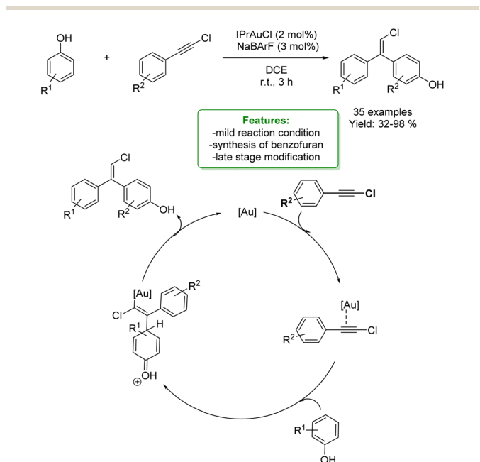
Scheme 63 Au-catalysed alkenylation of phenols with chloroalkyne. 183
