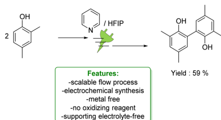
Scheme 89 Electrosynthesis of aryated phenols with arenes. 227-229
