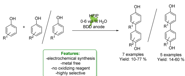
Scheme 88 Electrosynthesis of aryated phenols with arenes. 227-229
