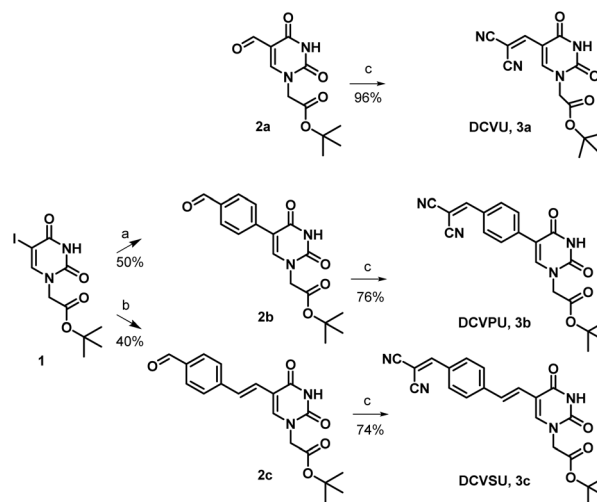
Scheme 1 Reagents and conditions (a) 4-formylphenylboronic acid, K 2 CO 3 , Pd(dppf)Cl 2 , THF/H 2 O (4 : 1), 100 °C, 5 h, (b) (4-formylstyryl) boronic acid, K 2 CO 3 , Pd(dppf)Cl 2 , THF/H 2 O (4 : 1), 100 °C, 5 h, (c) malononitrile, EtOH, 50 °C, 16 h.
