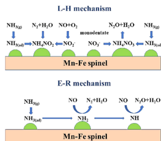
Fig. 14 Schematic diagram of the coexistence of L-H and E-R mechanisms on Mn-Fe spinel catalyst (reproduced from ref. 116 with permission from ACS Publications).
