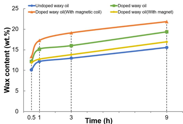
Fig. 8 Wax content of the doped waxy oil in the deposition layer under different magnetic treatments.
