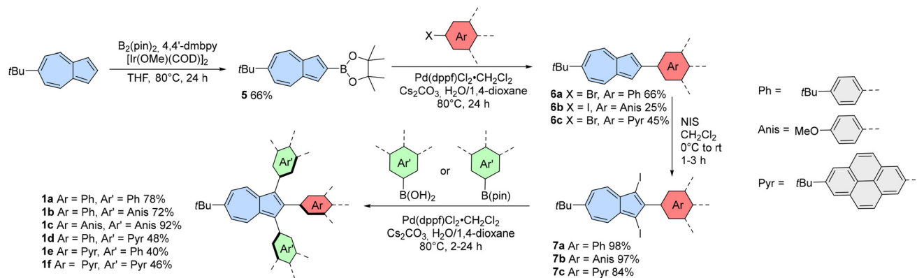
Scheme 2 Synthesis of azulene-containing precursors 1 . B 2 (pin) 2 = bis(pinacolato)diboron, 4,4'-dmbpy = 4,4'-dimethyl-2,2'-dipyridyl, COD = 1,5-cyclooctadiene, THF = tetrahydrofuran, dppf = 1,1'-bis(diphenylphosphino)ferrocene, NIS = N -iodosuccinimide.
