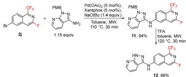
Scheme 9 Synthesis of valigilurax analogue 12 .
