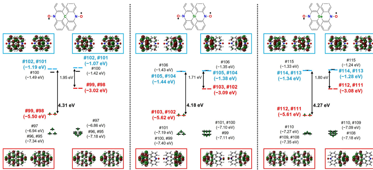
Fig. 5 Selected MO energy-level diagram for (left column) α and (right column) β spins in the triplet state for (left) SBDO-C, (centre) -Si and (right) -Ge. The MO images are superposed with an isovalue of 0.03. The red and blue MOs represent SOMOs and the lowest degenerate π* orbital, respectively.
